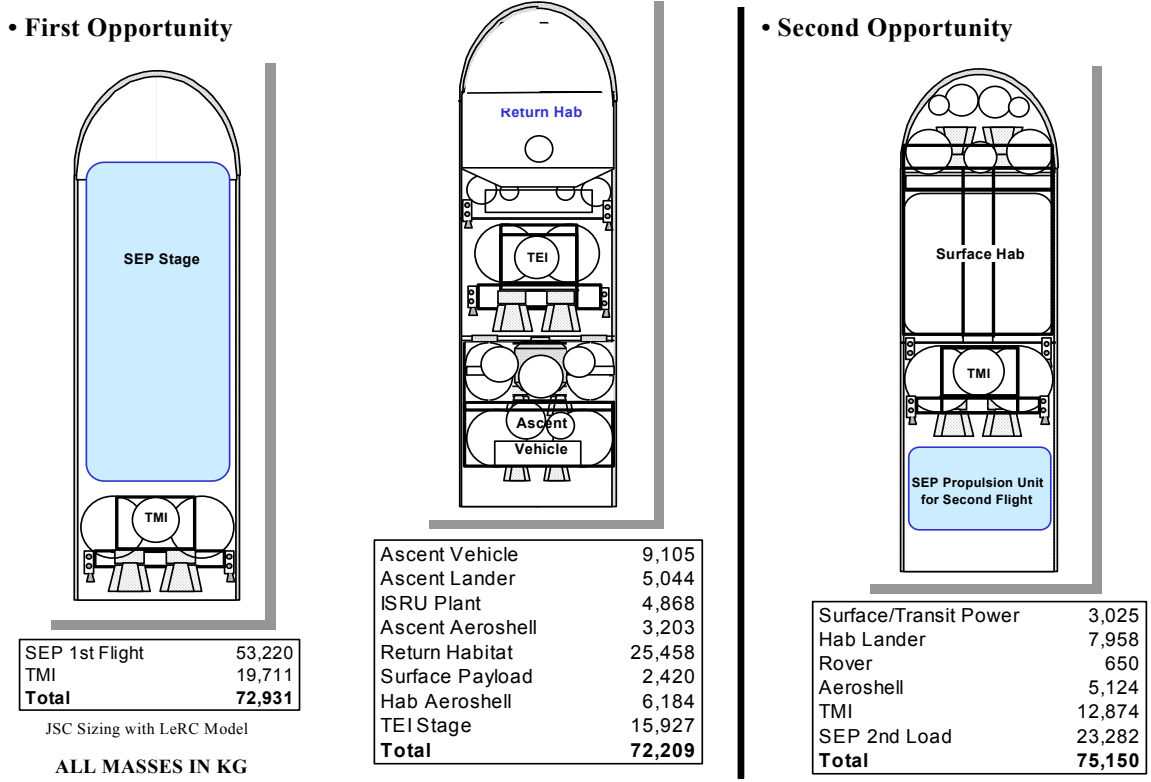
Figure A5-13 Three-Magnum Split Mission Launch Packages
