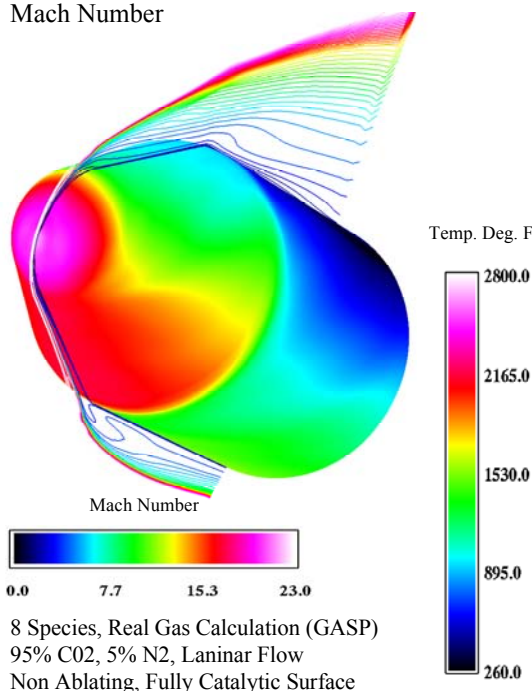
Figure A3-5 Aeroassist Study Results for Version 3.0
